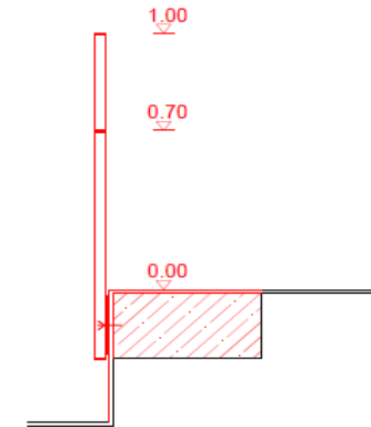
Detail (M=1:10)
