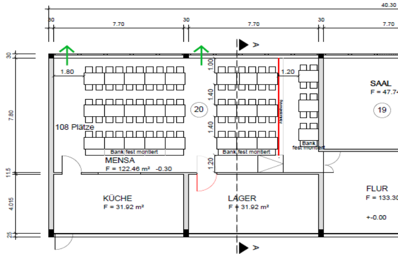
Grundriss (M=1:100)
